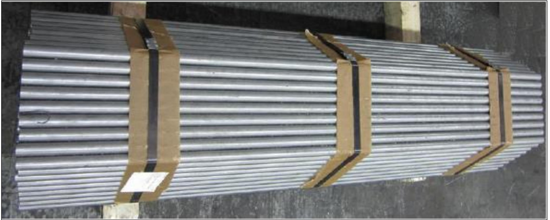
<Hexagonal packing>
